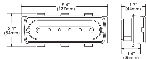
Linear 500 Series
