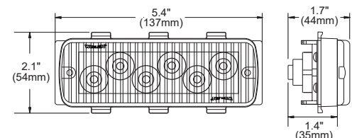
TIR6 500 Series
